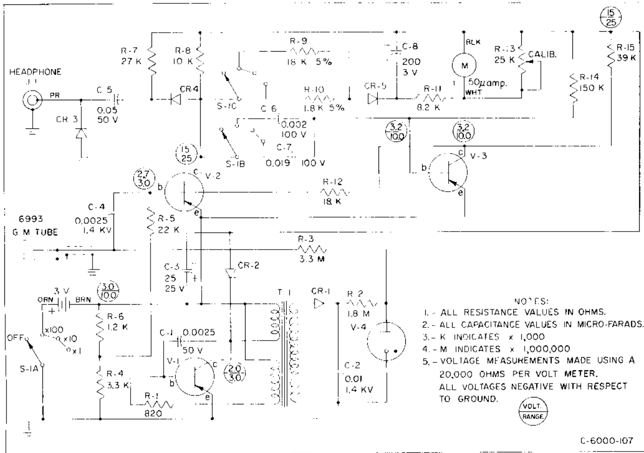
Fig. 5 — Schematic for V-700
