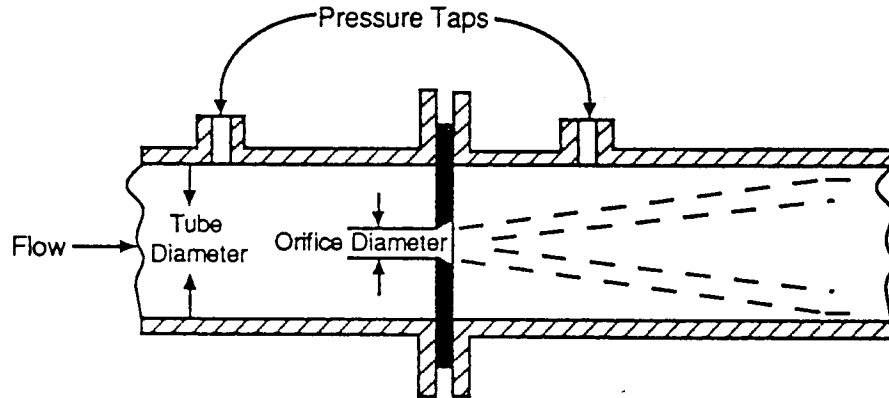
Figure 5.2. Orifice Meter
