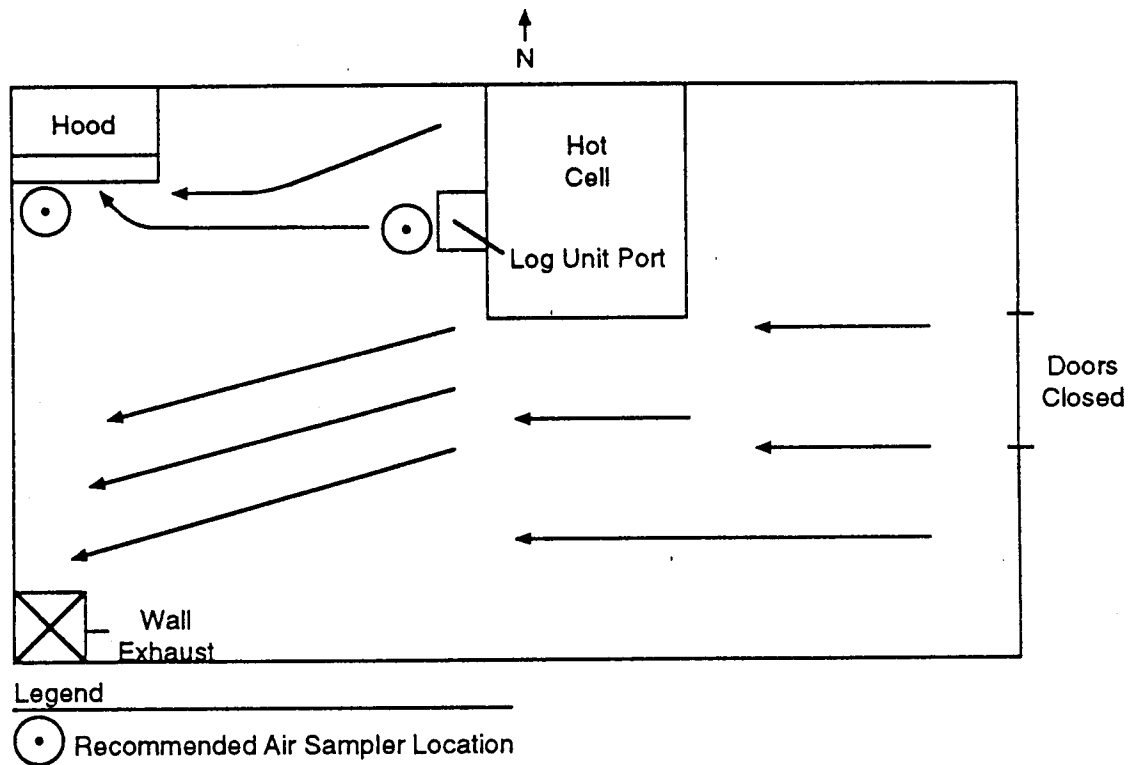
Figure 2.12. Example Work Area, Multiple Release Points in a New Facility
